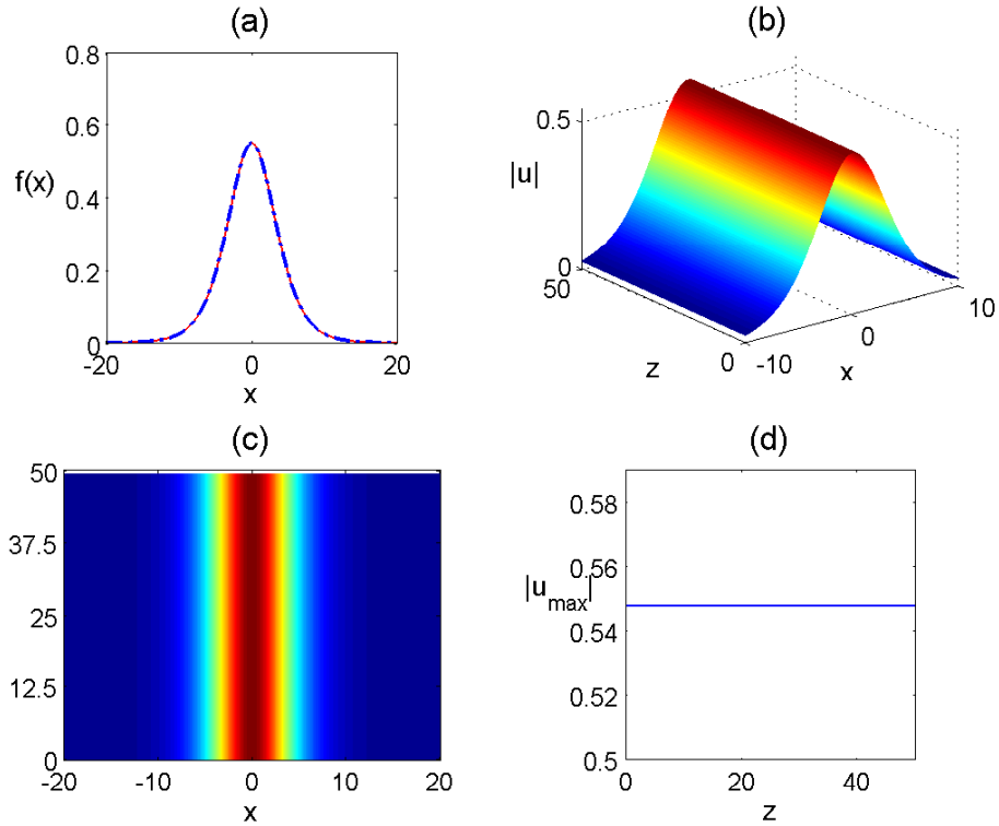
Figure 3.6 : Nonlinear stability of a higher order soliton for \gamma = -1, \mu = 0.16 ; (a) Numerically produced higher order soliton (blue dashes) on top of the solution after the evolution (red solid), (b) Nonlinear evolution of the soliton, (c) The view from top and (d) Maximum amplitude as a function of the propagation distance z .
